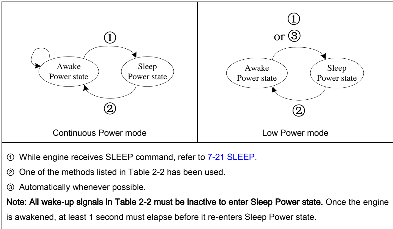
Figure 2-4 State machine of power management
