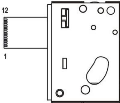
Figure 2-1 Top view
