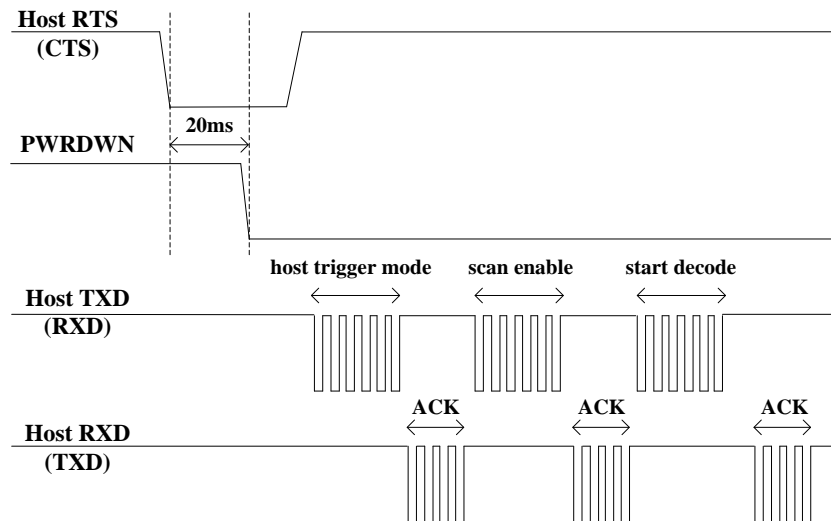
Figure 5-4 STRAT_DECODE timing
