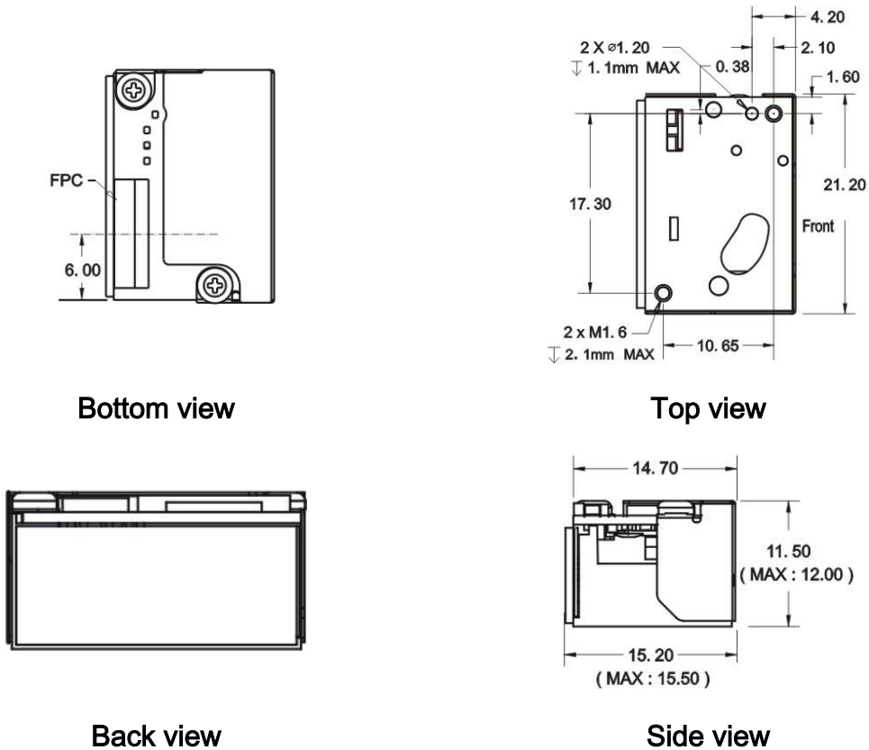
Figure 3-1 Mounting diagram
